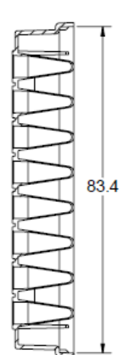
SECTION C-C
